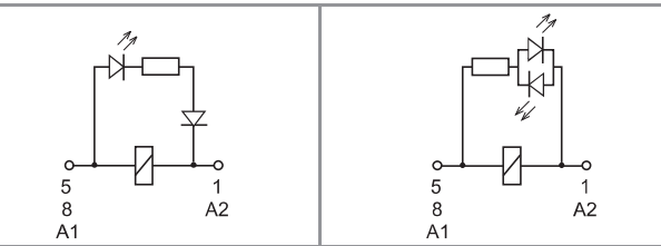
C: Option 54 LED (AC)
